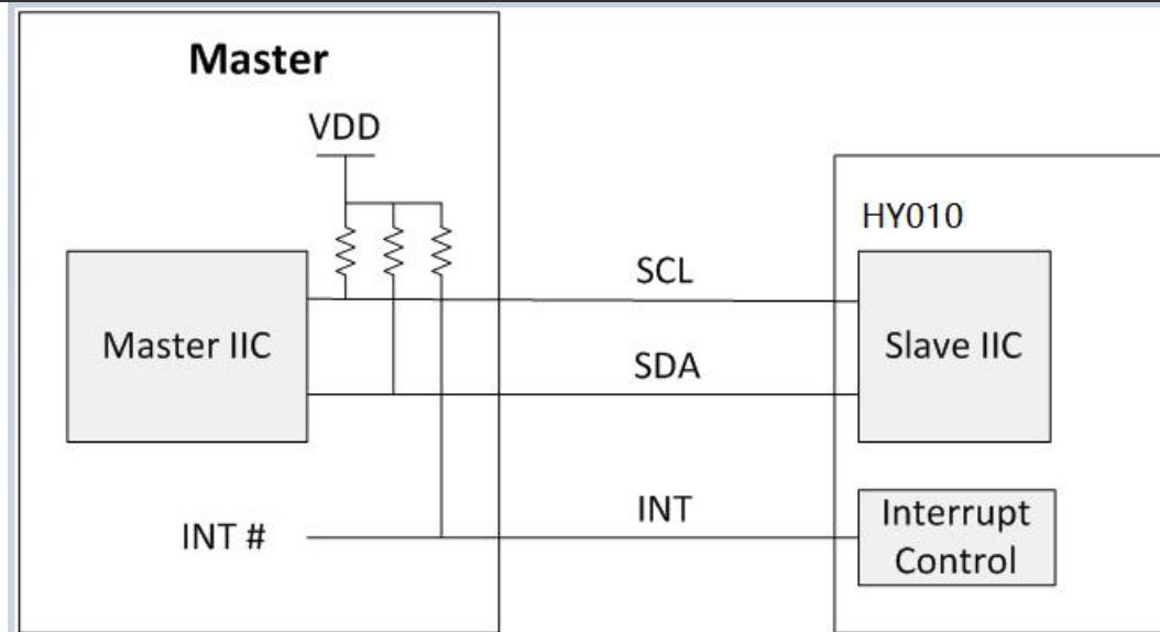
Figure6. IIC connect for master and HY010
