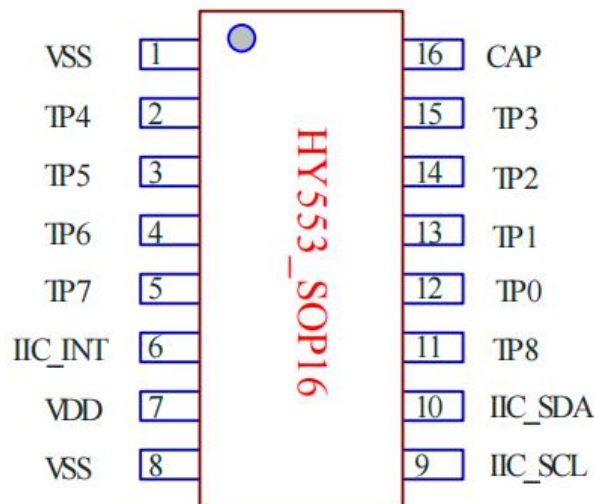
Figure5. pin define for IC package
