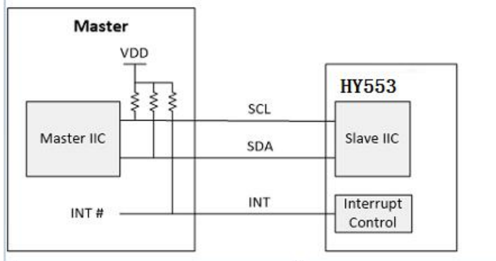
Figure6. IIC connect for master and HY553
