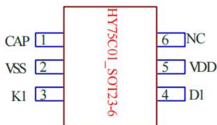
HY75C01 SOT-23-6
